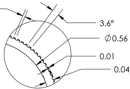
DETAIL A SCALE 4:1
